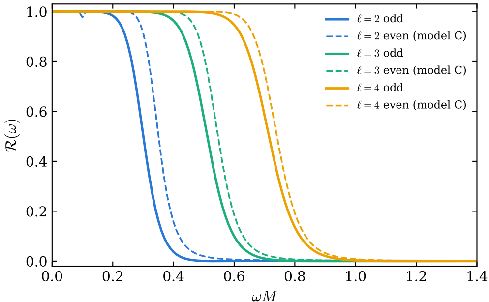
Shell at R = 3M : higher multipoles see a higher barrier
